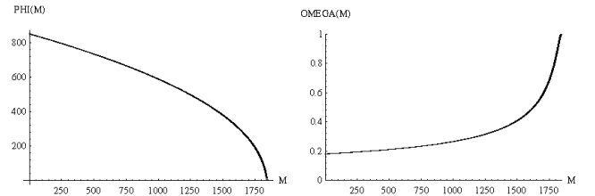
Figure 1: Average vocabulary size \Phi_{K_{\text{wiz}}}(M) and average OOV-rate \omega_{K_{\text{wiz}}}(M) depending on M
